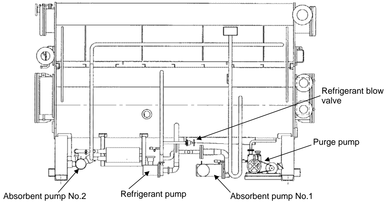
EVAPORATOR SIDE
