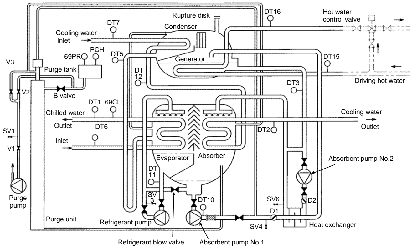
FLOW DIAGRAM
